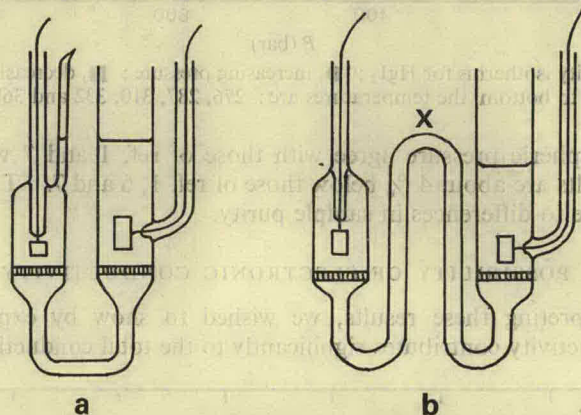
FIG. 7.—Cells used for electrolysis experiments on fused \text{HgI}_2 .
